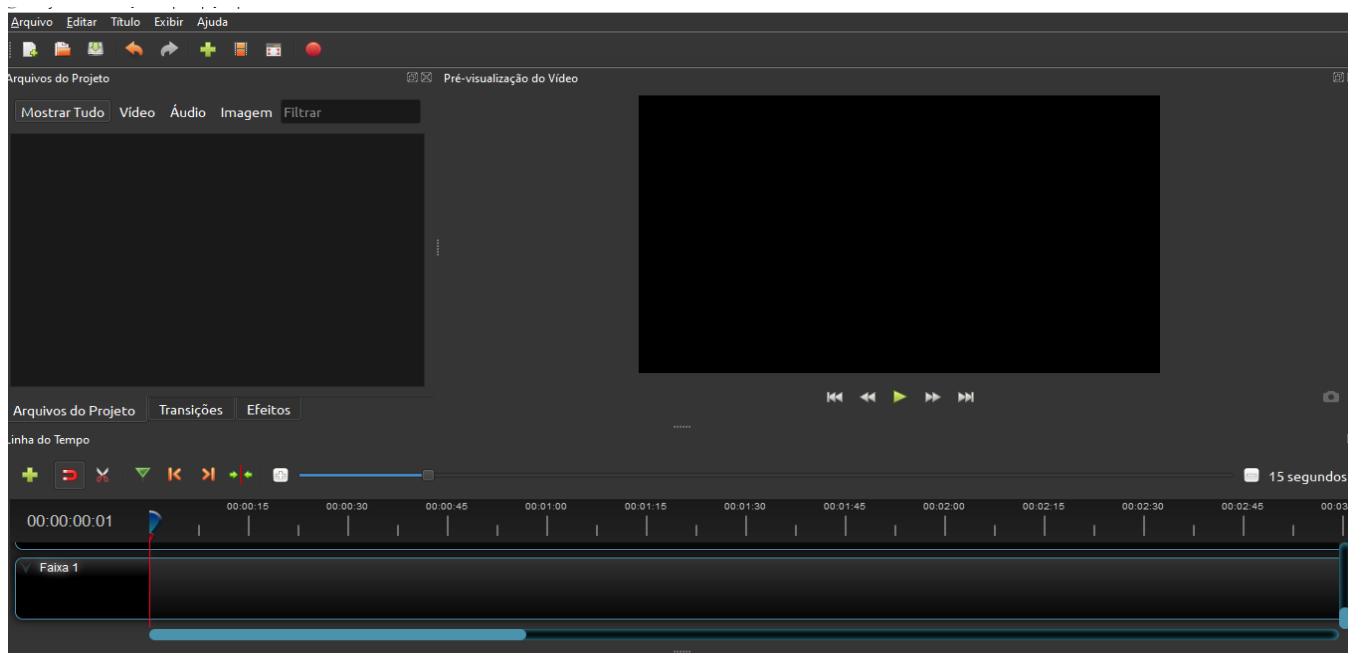
Figura 1 – OpenShot
